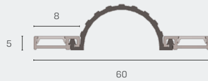
IS9050 Finger Guard Seal - hinge position
