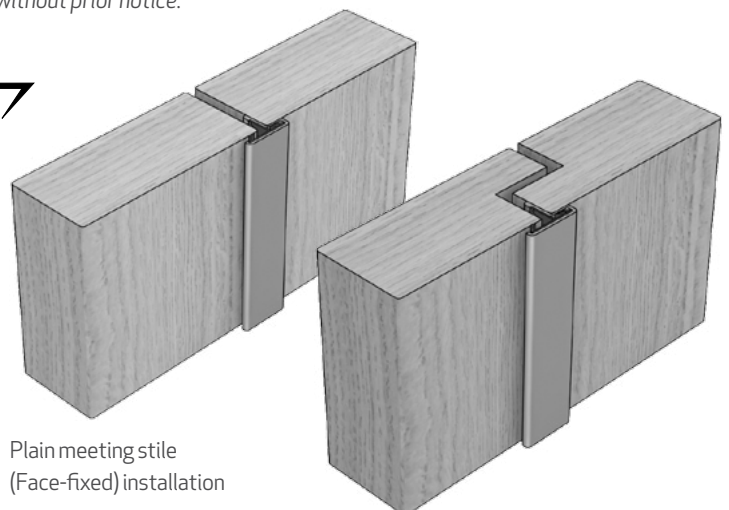
Rebated meeting stile installation
