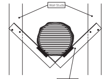
Guard Removed for clarity FACE FIXING Alternative fixing method Kilargo Intumescent fire damper supported by external Rondo angle hurrin between studs
