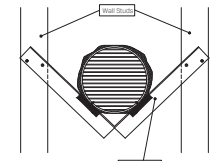
Guard Removed for clarity FACE FIXING Alternative fixing method Kilargo Intumescent fire damper supported by external Rondo angle built between studs
